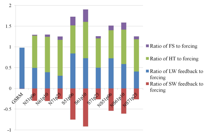
Fig. 9. Changes in the atmospheric energy balance in the region where the solar reduction was imposed, normalized by the region's reduction in short-wave radiative forcing. The terms shown are for the net change in the surface-to-atmosphere heat flux (FS), the atmospheric horizontal heat flux into the region (HT), the net long-wave energy flux (LW), and the net change in short-wave radiation (SW).
